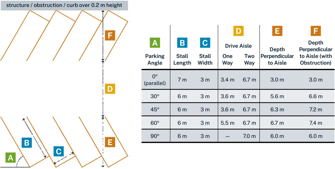
FIGURE 17 — Parking Facility Dimensions
