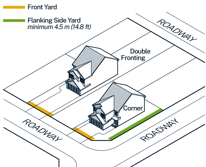
FIGURE 6 — Corner and Double Fronting Parcels
