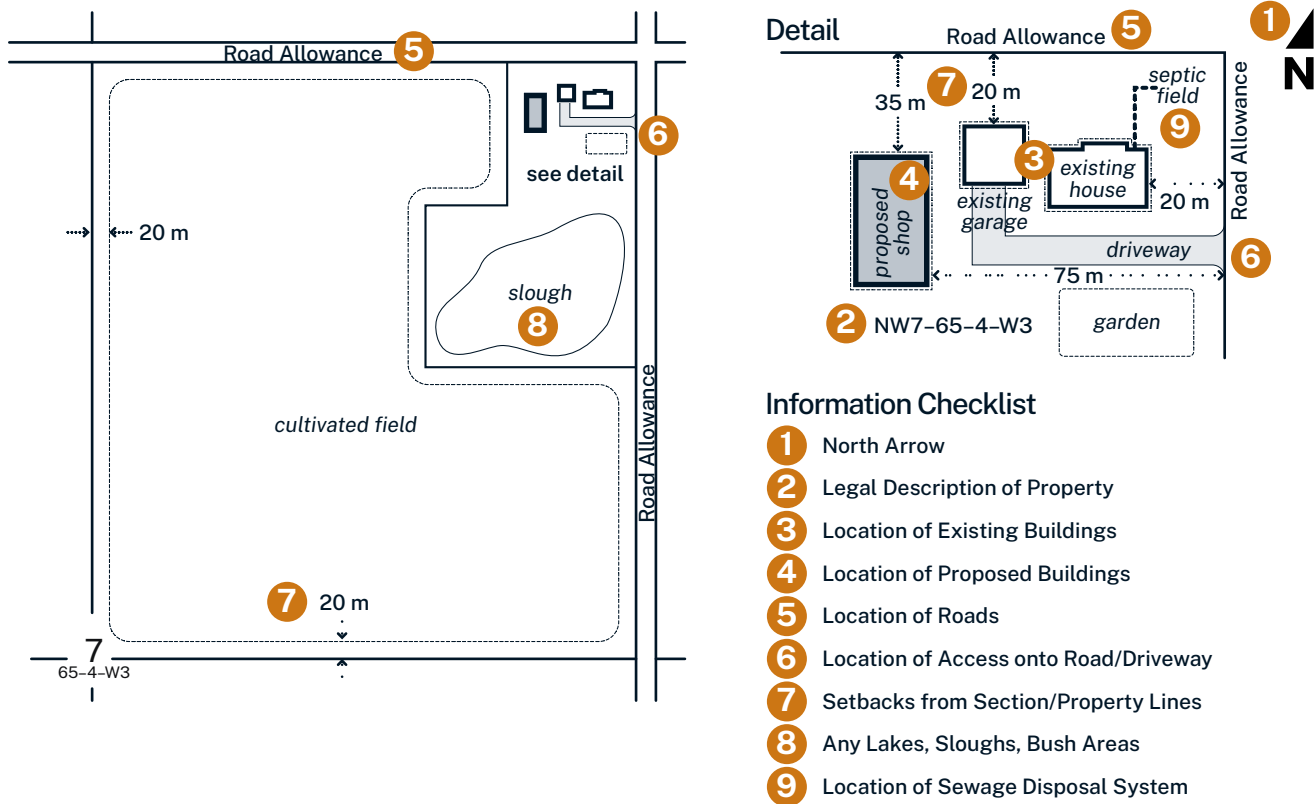
FIGURE 1 — Sample Rural Site Plan
